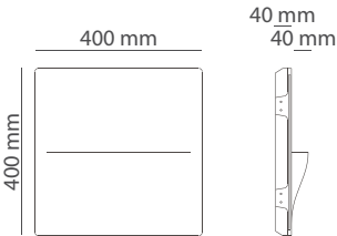
Dimensione foro 403x403 mm Cut hole sizes 403x403 mm
