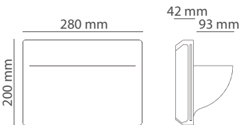
Dimensione foro 283x203 mm Cut hole sizes 283x203 mm
