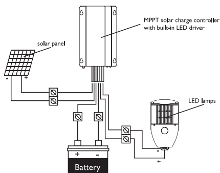
PARTS CONNECTION DIAGRAM
